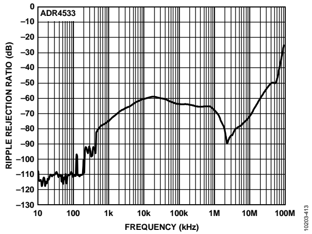
Figure 52. ADR4533 Ripple Rejection Ratio vs. Frequency
