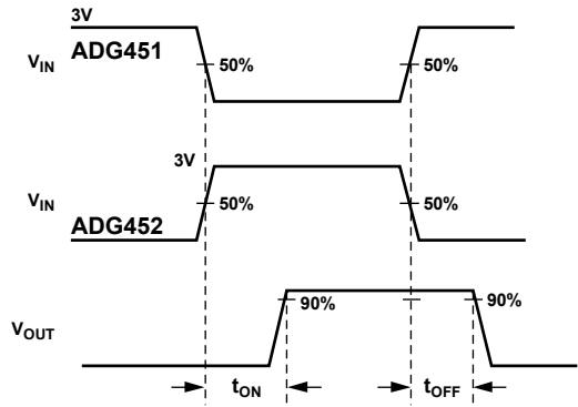
Figure 19. Switching Times
