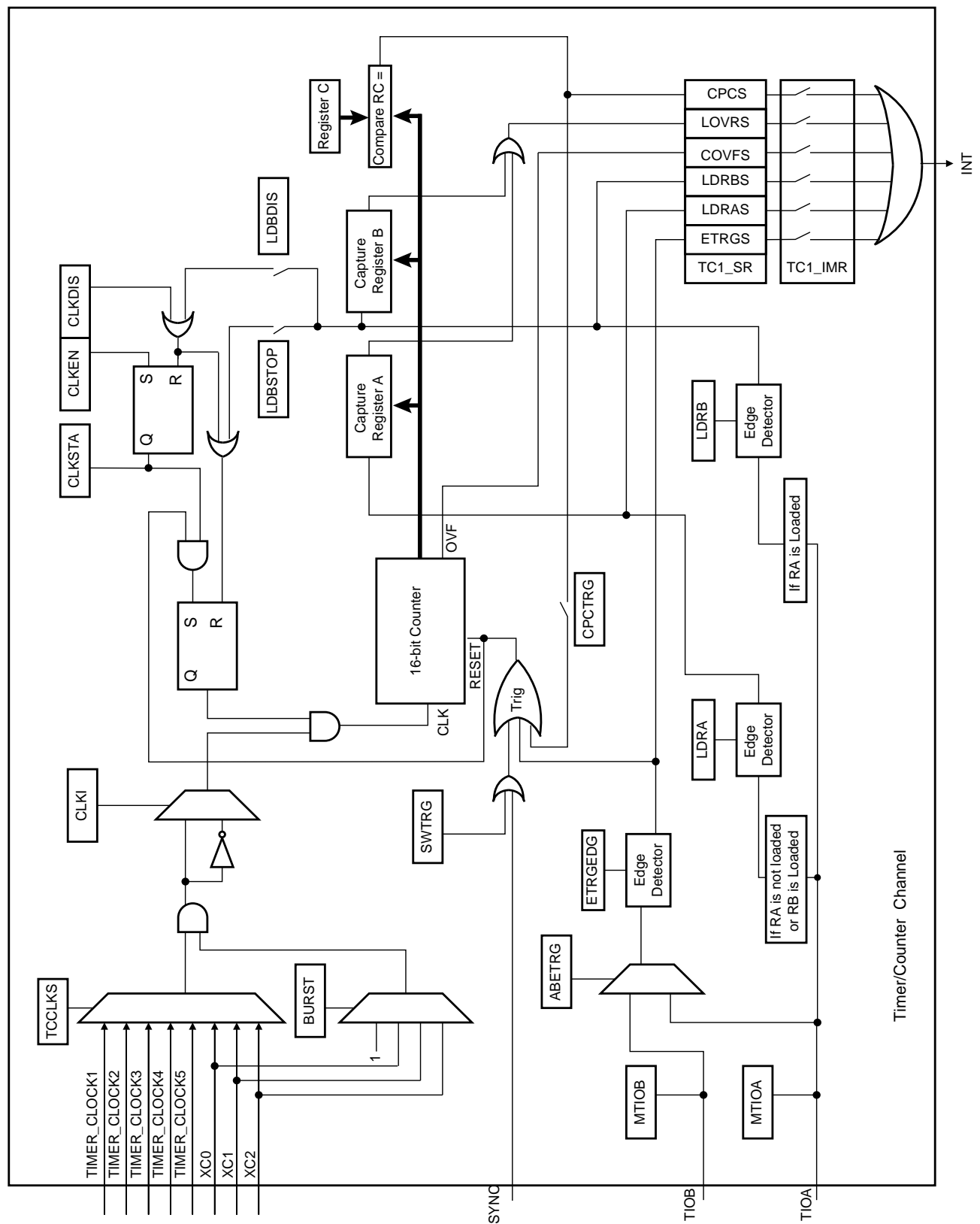
Figure 33-5. Capture Mode
