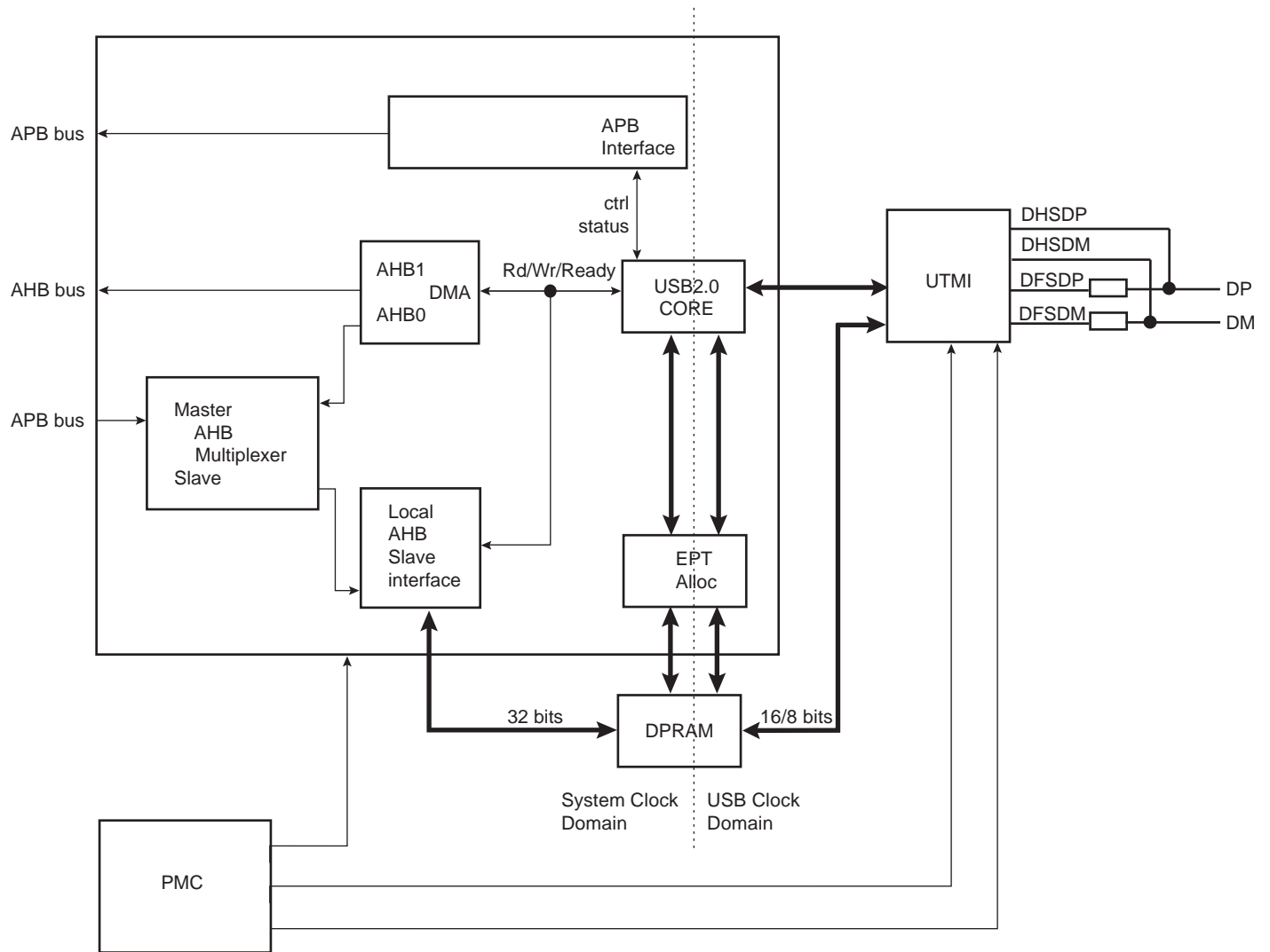
Figure 39-2. Block Diagram
