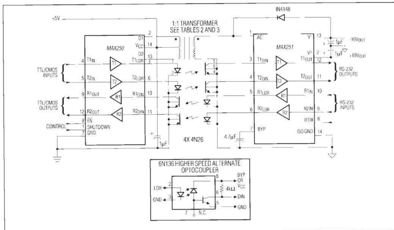
Figure 3. Isolated RS-232 Interface
