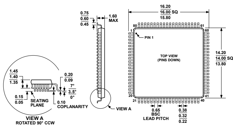
Figure 62. 80-Lead Low Profile Quad Flat Package [LQFP] (ST-80-2)
