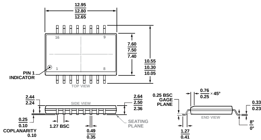
Figure 26. 16-Lead Standard Small Outline Package, with Increased Creepage [SOIC_IC] Wide Body (RW-16-2)
