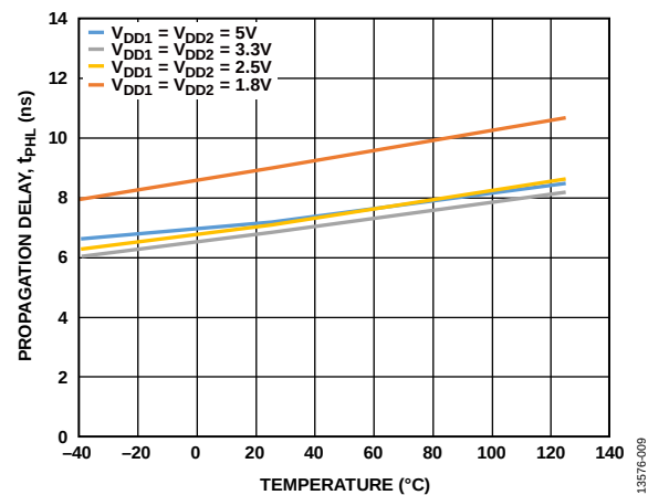
Figure 18. Propagation Delay, t_{PHL} vs. Temperature at Various Voltages
