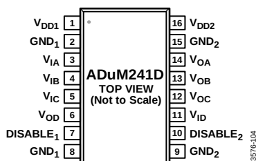
Figure 7. ADuM241D Pin Configuration
