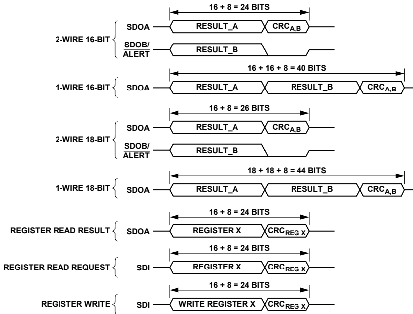
Figure 43. CRC Operation
