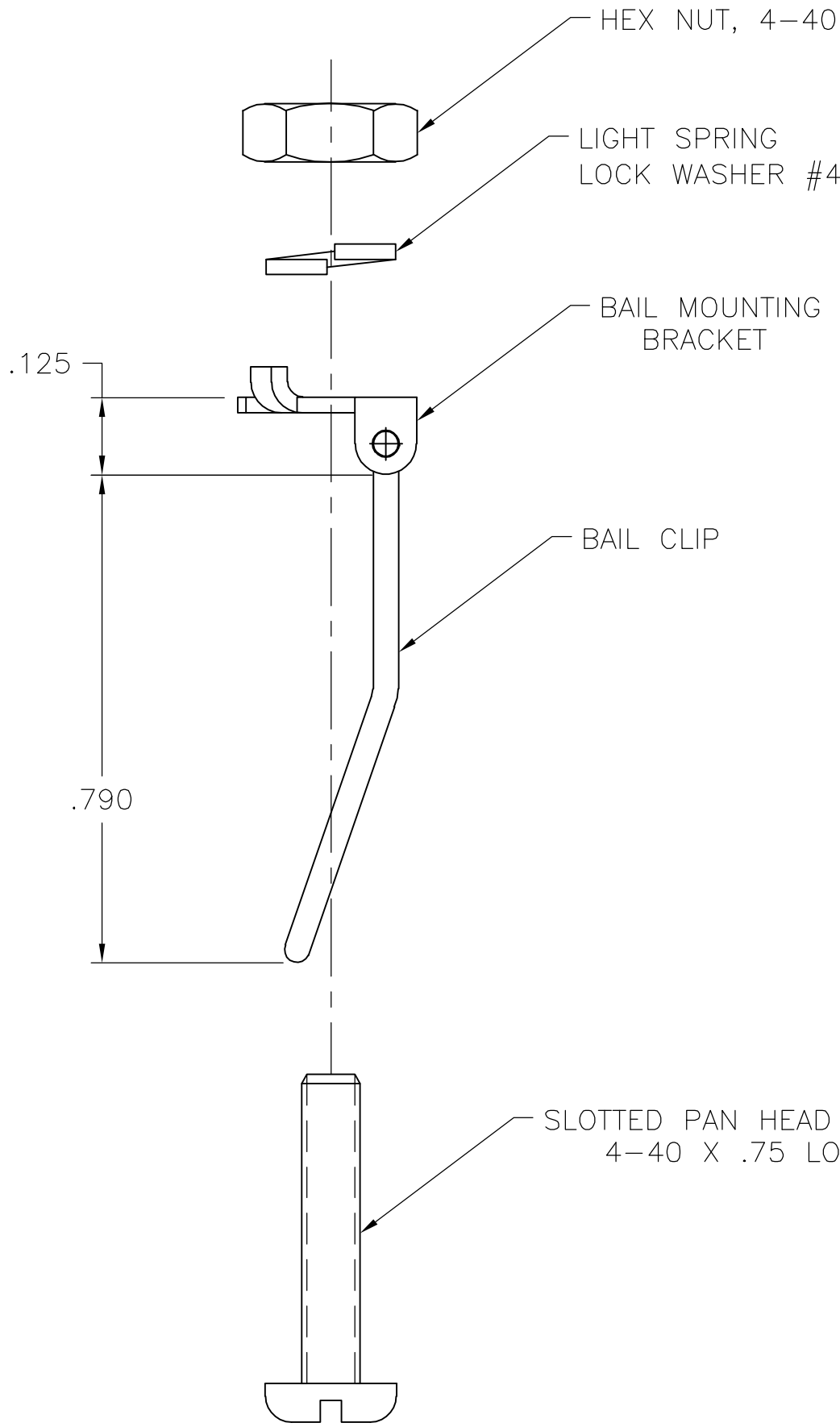
KIT P/N 5552562-1 VIEW A
