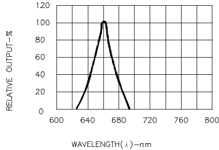
Fig.1 SPECTRAL RESPONSE
