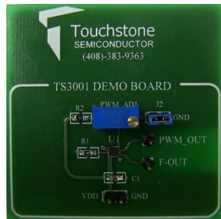
Figure 2. TS3001 Evaluation Board
