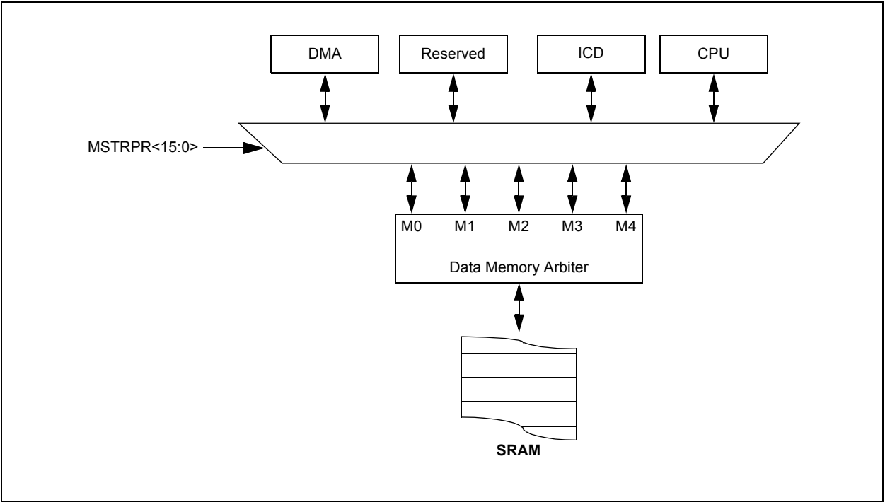
FIGURE 4-18: ARBITER ARCHITECTURE
