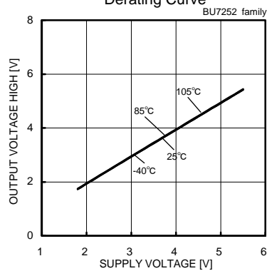
Fig. 27 Output Voltage High – Supply Voltage (RL=10[kΩ])
