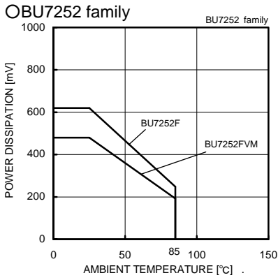
Fig. 23 Derating Curve
