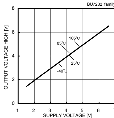
Fig. 71 Output Voltage High – Supply Voltage (RL=10[kΩ])
