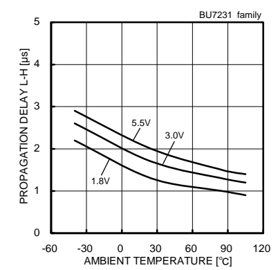
Fig. 65 Propagation Delay L-H – Ambient Temperature
