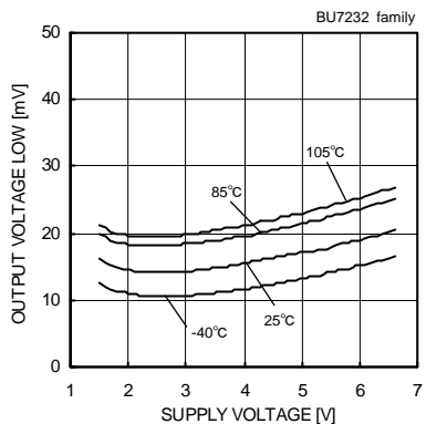
Fig. 73 Output Voltage Low – Supply Voltage (RL=10[kΩ])
