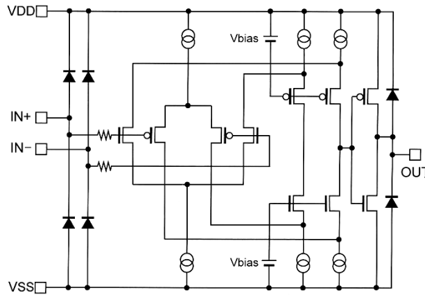
Fig. 89 Simplified schematic
