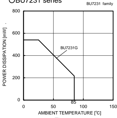
Fig. 45 Derating Curve
