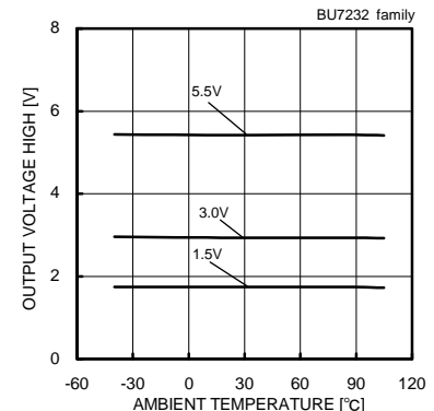
Fig. 72 Output Voltage – Ambient Temperature (RL=10[kΩ])
