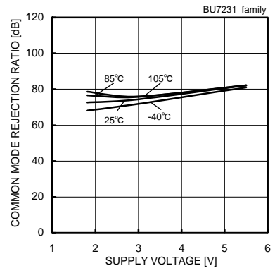
Fig. 62 Common Mode Rejection Ratio – Supply Voltage (VDD=3[V])
