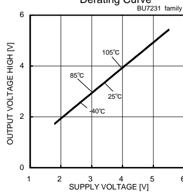
Fig. 49 Output Voltage - Supply Voltage ( R_L=10[k\Omega] )
