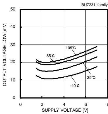
Fig. 51 Output Voltage Low - Supply Voltage ( R_L=10[k\Omega] )
