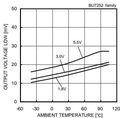
Fig. 30 Output Voltage Low – Ambient Temperature(RL=10[kΩ])
