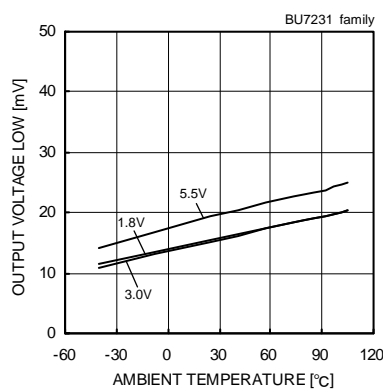
Fig. 52 Output Voltage Low - Ambient Temperature ( R_L=10[k\Omega] )
