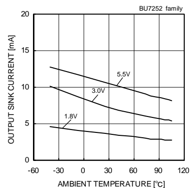
Fig. 34 Output Sink Current - Ambient Temperature (VOUT=VSS+0.4[V])
