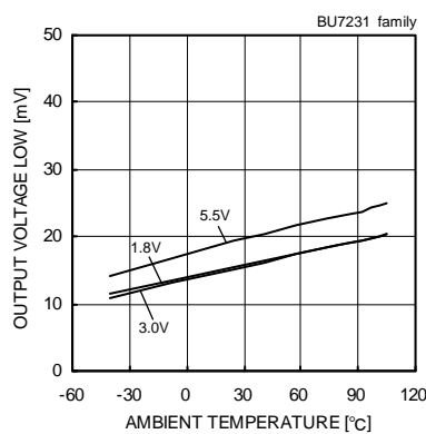
Fig. 52 Output Voltage Low - Ambient Temperature ( R_L=10[k\Omega] )
