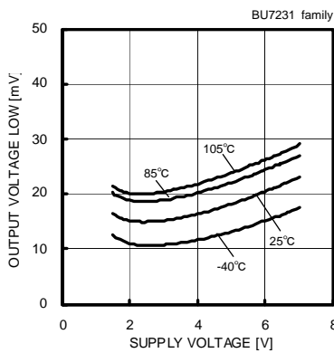
Fig. 51 Output Voltage Low - Supply Voltage ( R_L=10[k\Omega] )
