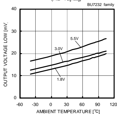
Fig. 74 Output Voltage Low - Ambient Temperature ( R_L=10[k\Omega] )
