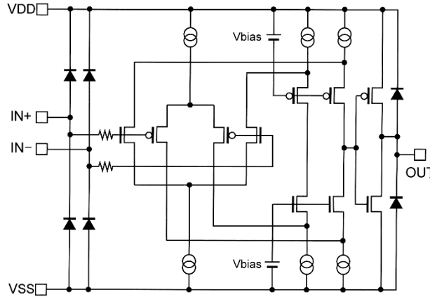
Fig. 89 Simplified schematic
