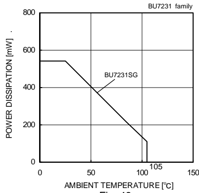
Fig. 46 Derating Curve
