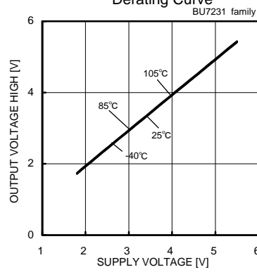
Fig. 49 Output Voltage - Supply Voltage ( R_L=10[k\Omega] )
