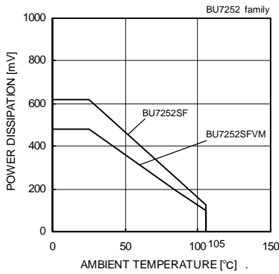
Fig. 24 Derating Curve
