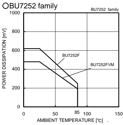
Fig. 23 Derating Curve
