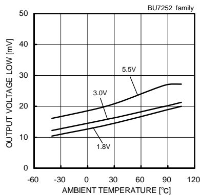
Fig. 30 Output Voltage Low – Ambient Temperature(RL=10[kΩ])
