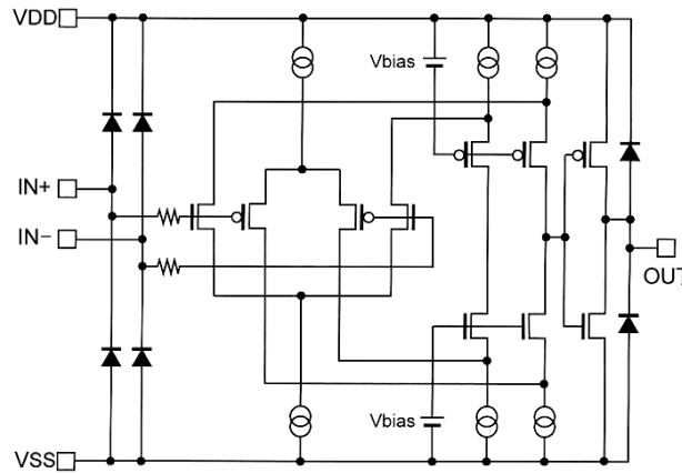
Fig. 89 Simplified schematic
