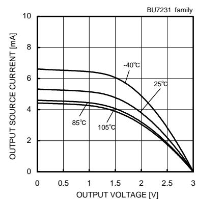
Fig. 53 Output Source Current - Output Voltage ( V_{DD}=3[V] )
