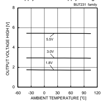
Fig. 50 Output Voltage High - Ambient Temperature ( R_L=10[k\Omega] )
