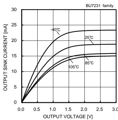
Fig. 55 Output Sink Current - Output Voltage ( V_{DD}=3[V] )
