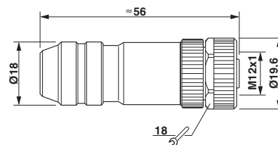
Dimensioned drawing
