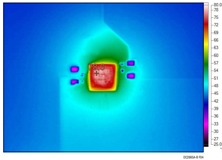
Figure 4. Measured Thermal Capture at 12V IN and 1.5V OUT , 15A OUT at 25°C Ambient with No Airflow
