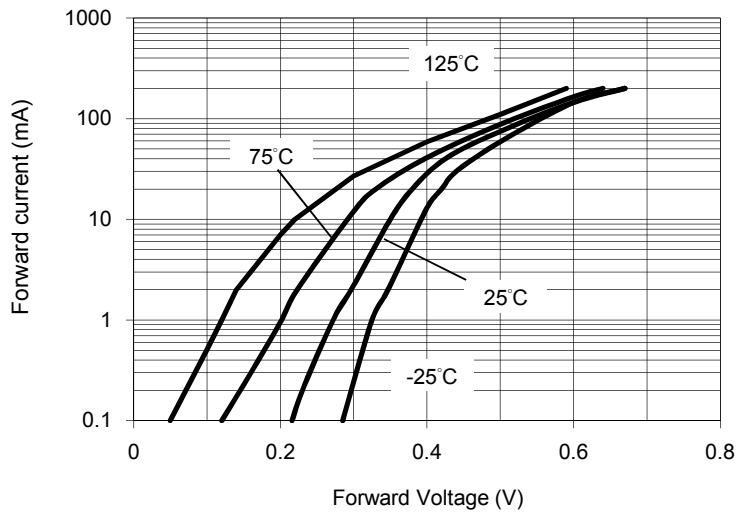
Fig.1 Forward Characteristics
