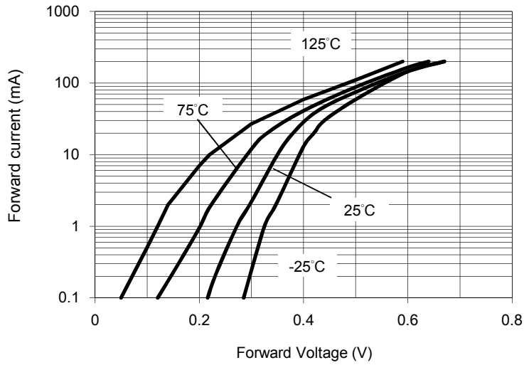
Fig.1 Forward Characteristics
