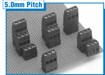
5.0mm Pitch ESMT Multi-tier . . . . . Pages 70-71 17.5A / 300V
