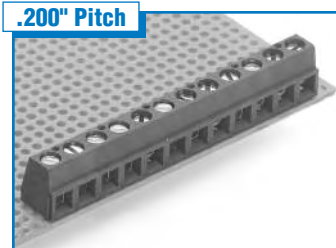
.200" Pitch ESLM Low-Profile, R/A . . . Page 65 13.5A / 300V
