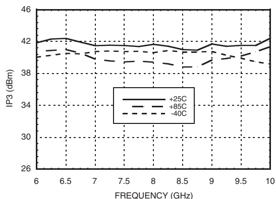
Output IP3 vs. Temperature 7V @ 940 mA, Pin/Tone = -15 dBm
