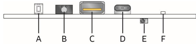
Figure 9. Front Panel Connectors, Controls and Indicators
