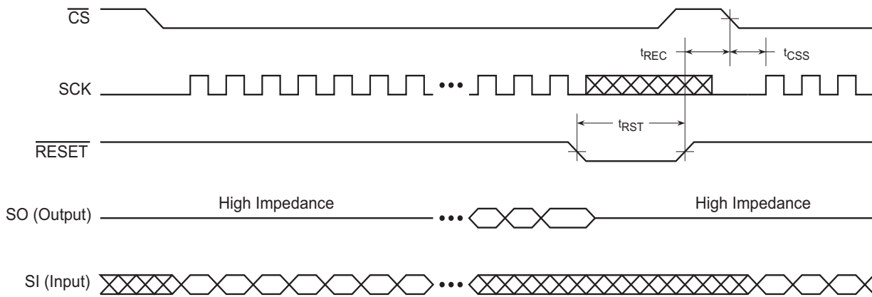
Figure 24-12. Reset Timing
