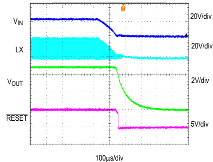
SHUTDOWN THROUGH INPUT SUPPLY VIN = 24V, VOUT = 5V, IOUT = 1.7A, MODE = SGND
