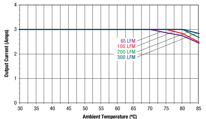
Maximum Current Temperature Derating at Sea Level (V IN = 24V, V OUT = 15V, transverse airflow)
