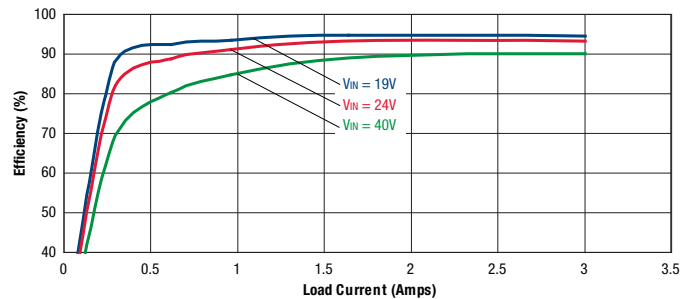
Efficiency vs. Line Voltage and Load Current @ +25°C (V OUT = 12V)
