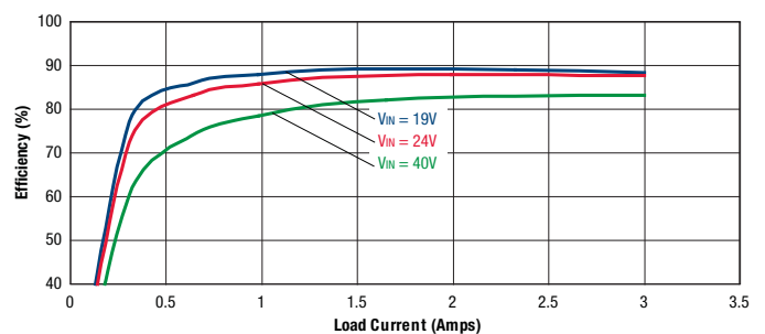
Efficiency vs. Line Voltage and Load Current @ +25°C (V OUT = 5V)
