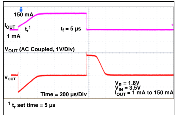
FIGURE 2-53: Dynamic Load Response.
