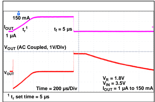
FIGURE 2-52: Dynamic Load Response.
