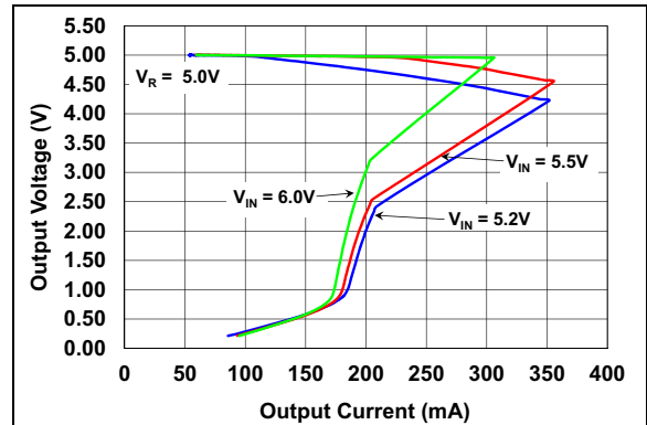
FIGURE 2-24: Output Voltage vs. Output Current.
