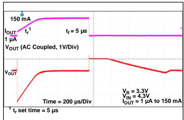
FIGURE 2-54: Dynamic Load Response.
