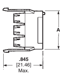
Cap Rear
