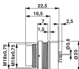
Dimensional drawing
