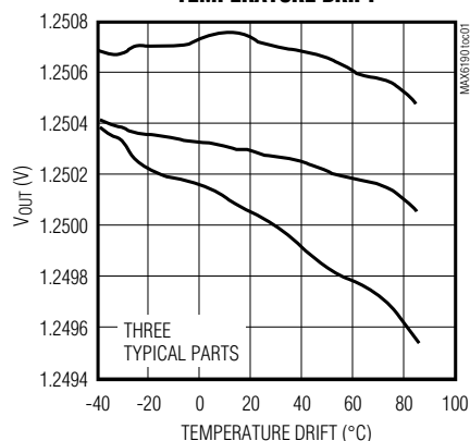
MAX6190 OUTPUT VOLTAGE TEMPERATURE DRIFT
