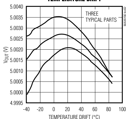
MAX6195 OUTPUT VOLTAGE TEMPERATURE DRIFT
