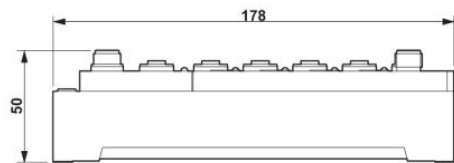
Dimensioned drawing
