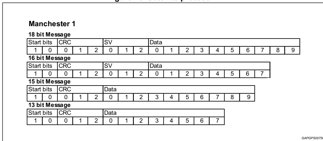
Figure 16. Satellite protocol-A
