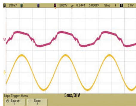
Figure 6. 230VAC (PF = 0.97)
