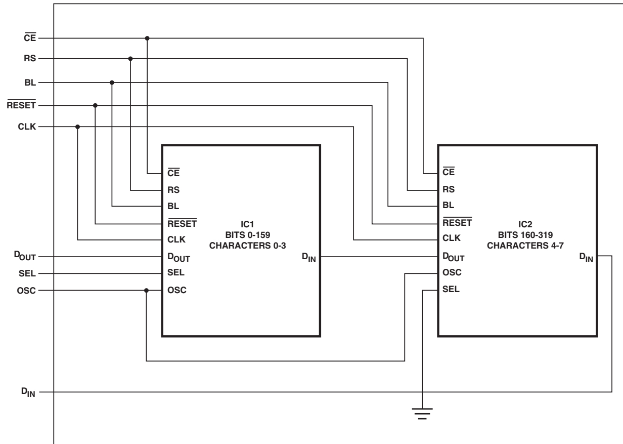
Figure 8. Cascaded ICs
