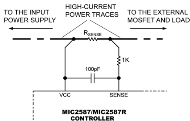
Figure 7. Current-Limit Sense Filter for Noisy Systems
