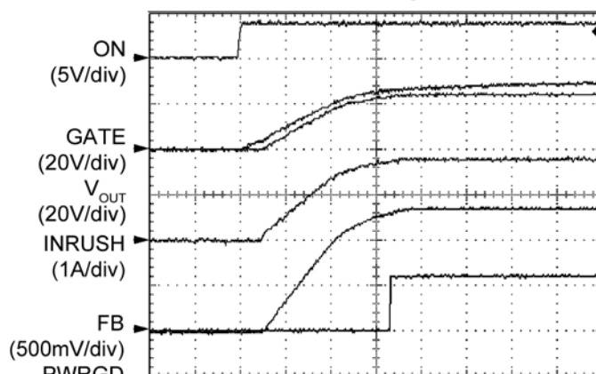
Turn-On Response
