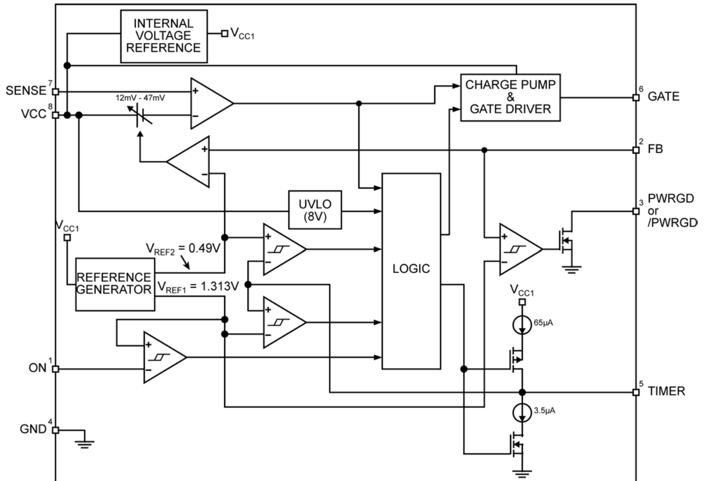
MIC2587/MIC2587R Block Diagram
