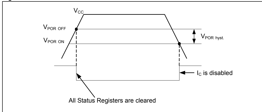
Figure 4. Power-on reset
