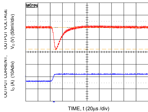
Figure 34. Transient Response to Dynamic Load Change from 50% to 100% at 12V in , C_{out}=5\mu\text{F} , C_{Tune}=1500\text{pF} & R_{Tune}=330\text{ohms}
