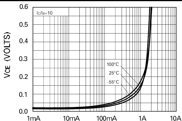
Collector Current V CE (SAT) vs I C
