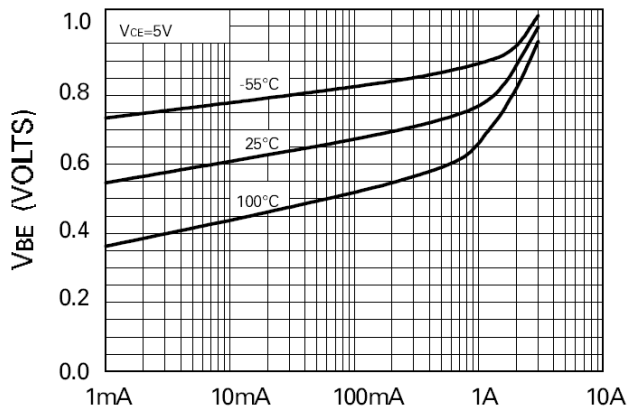
Collector Current V BE (ON) vs I C
