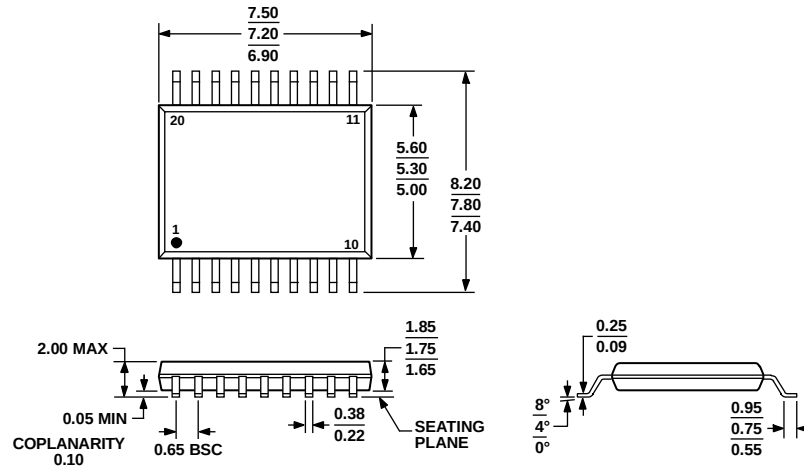
COMPLIANT TO JEDEC STANDARDS MO-150-AE Figure 3. 20-Lead Shrink Small Outline Package [SSOP] (RS-20) Dimensions shown in millimeters
