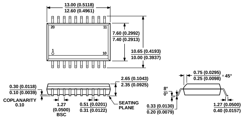
COMPLIANT TO JEDEC STANDARDS MS-013-AC CONTROLLING DIMENSIONS ARE IN MILLIMETERS; INCH DIMENSIONS (IN PARENTHESES) ARE ROUNDED-OFF MILLIMETER EQUIVALENTS FOR REFERENCE ONLY AND ARE NOT APPROPRIATE FOR USE IN DESIGN.
