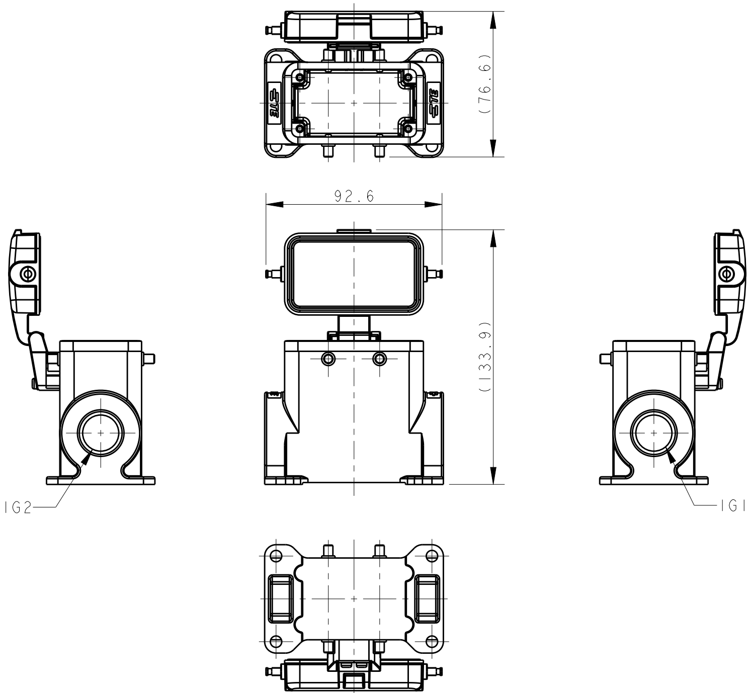
TYPE 2: HIGHT BODY + METAL PROTECTION COVER OTHER SPEC REFER TO TYPE 1
