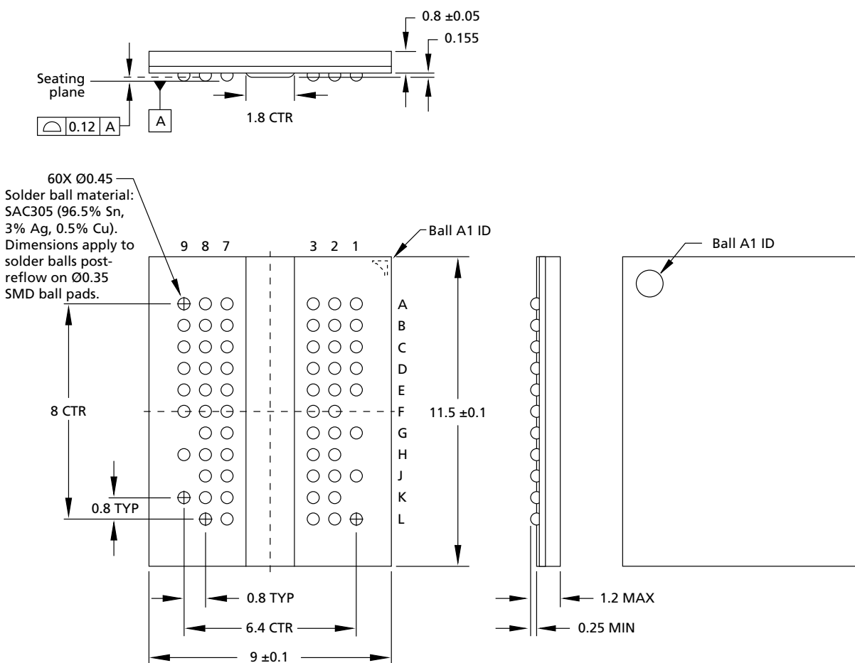
Figure 6: 60-Ball FBGA Package (9mm x 11.5mm) – x8
