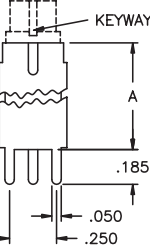
FRONT VIEW DOUBLE POLE
