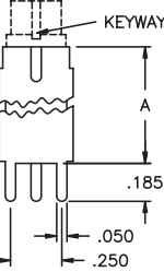
FRONT VIEW DOUBLE POLE
