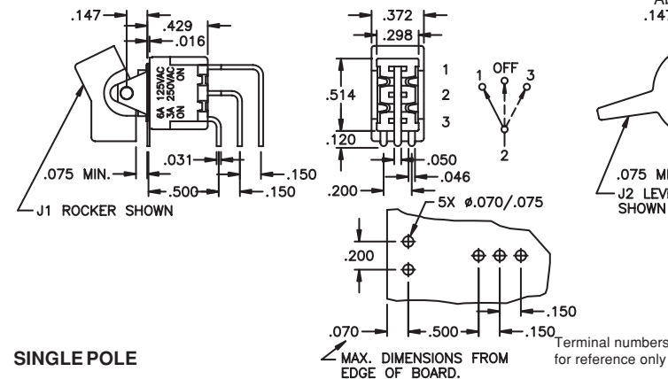
SINGLE POLE WITH J1 ROCKER
