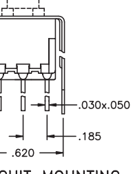
PRINTED CIRCUIT MOUNTING
