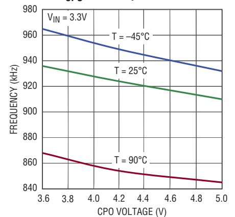
Charge Pump Oscillator Frequency vs V_{CPO} and Temperature
